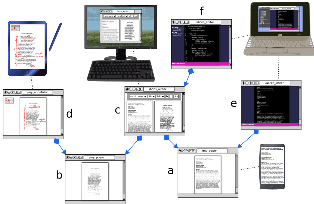
Figure 3 An example of a network of interconnected webstrates. The blue arrows are transclusions establishing application-document relationships. a) A paper, displayed on a mobile device. b) A poem. c) Bob’s word processor editing a and b on his desktop computer. d) Bob’s annotation webstrate which lets Bob hand-annotate webstrates with his tablet and stylus. e) Alice’s HTML markup editor, editing the paper a on her laptop. f) Alice’s script editor, extending Bob’s word processor on a different window of her laptop.
